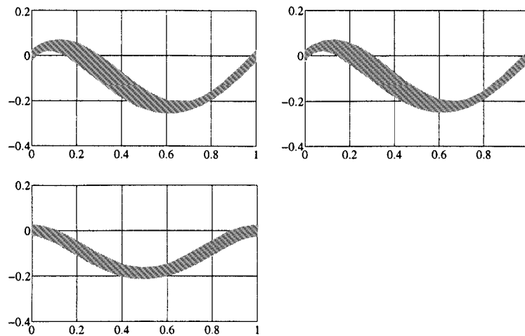
Figure 1. Deformation of the cross-section of a plate in plane strain as determined by the Reissner–Mindlin (top left), elastic (top right), and Kirchhoff–Love models (bottom), respectively.
