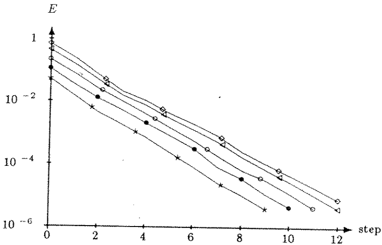
Fig. 5. Convergence history in the case of 16 subdomains
