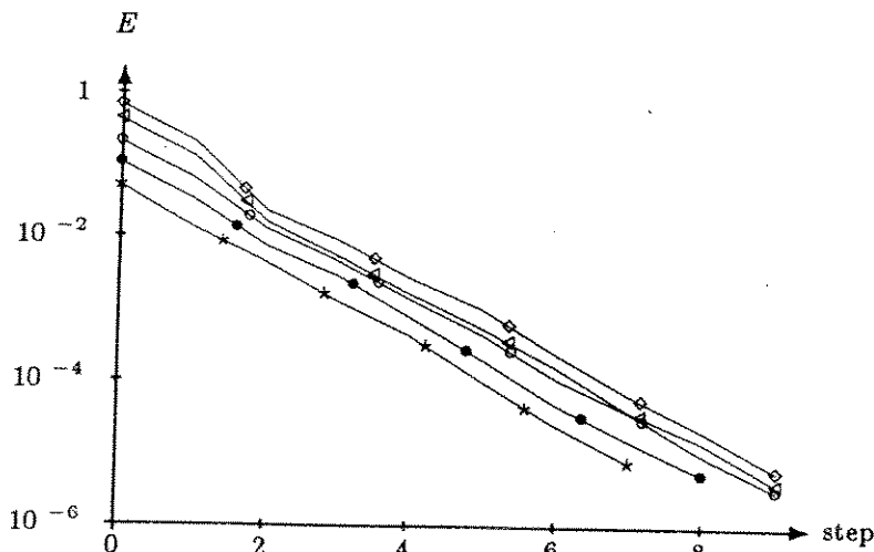
Fig. 4. Convergence history in the case of 4 subdomains \ast: h = \frac{1}{8}, \bullet: h = \frac{1}{16}, \circ: h = \frac{1}{32}, \triangleleft: h = \frac{1}{64}, \diamond: h = \frac{1}{100}
