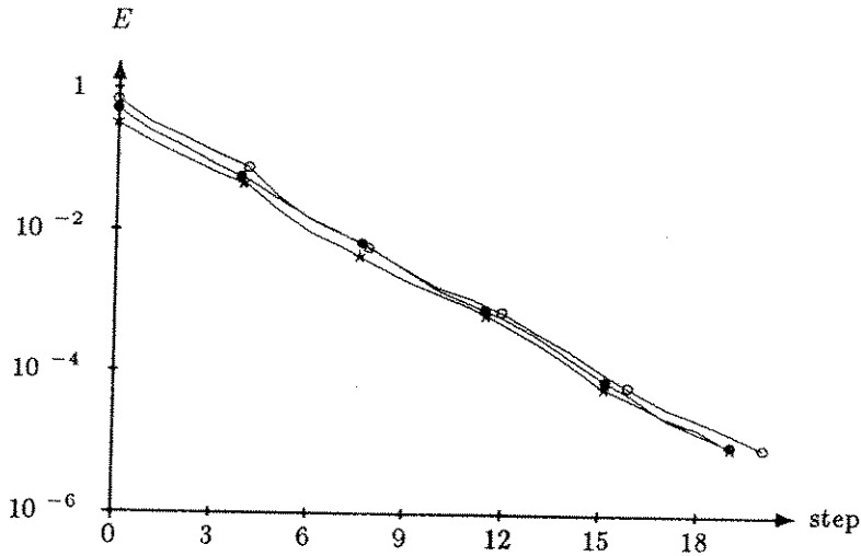
Fig. 6. Convergence history in the case of 64 subdomains.
