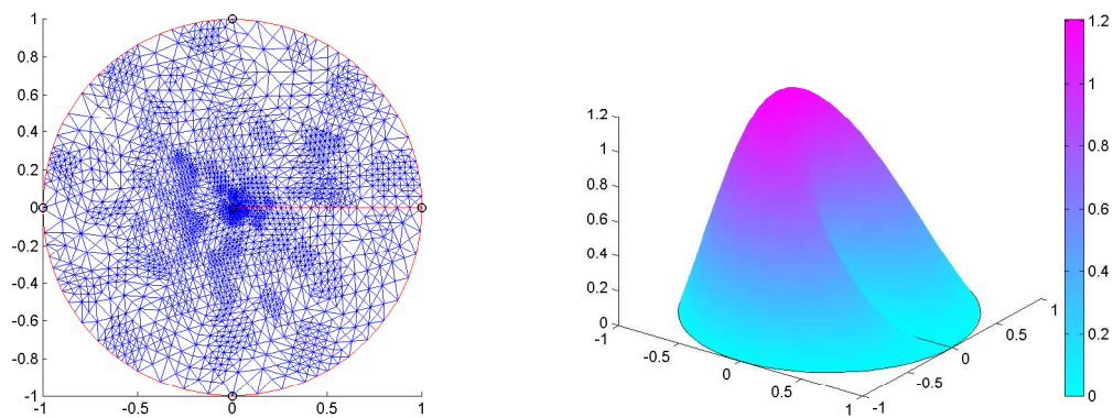
Figure 6. The adaptively refined mesh (left) of 6135 elements and the eigenfunction u_{1,7}^1 (right) after 7 adaptive iterations for Example 6.2
