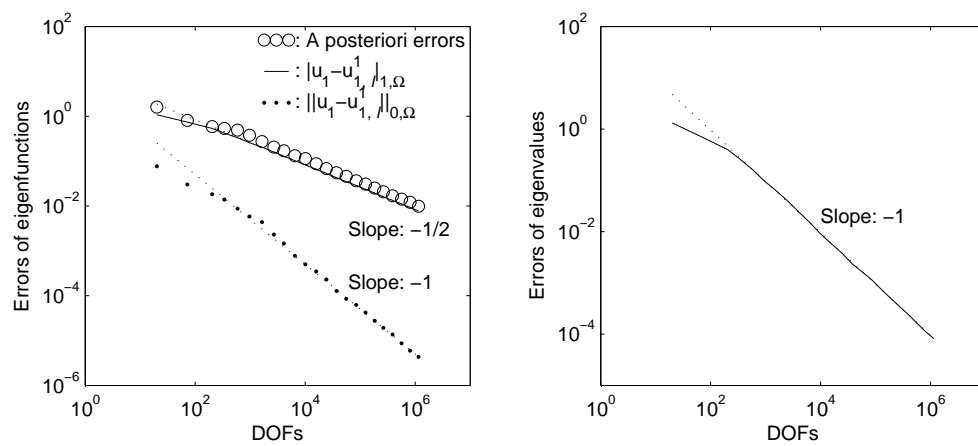
Figure 5. Convergence rates of u_{1,\ell}^1 (left) and \lambda_{1,\ell}^1 (right) for Example 6.2. Dotted lines give reference slopes.
