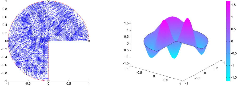
Figure 4. The adaptively refined mesh (left) of 7491 elements and the eigenfunction u_{10,8}^{10} (right) after 8 adaptive iterations for Example 6.1
