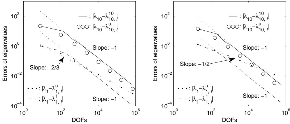
Figure 9. Convergence rates of \lambda_{10,\ell}^{10} , \lambda_{10,\ell}^u , \lambda_{1,\ell}^u and \lambda_{1,\ell}^1 for Example 6.1 (left) and for Example 6.2 (right). Dotted lines give reference slopes.
