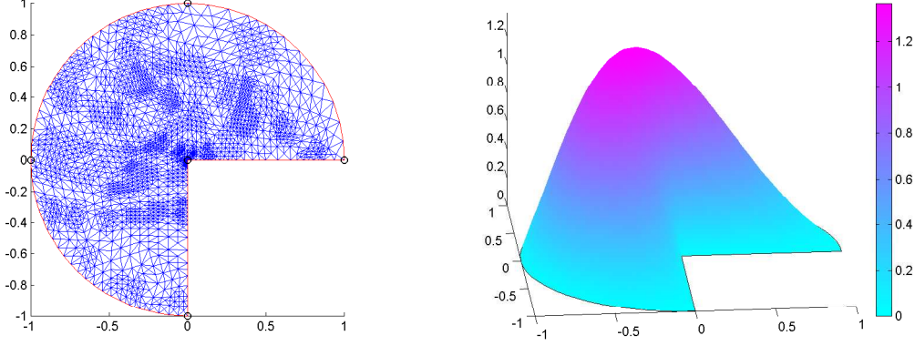
Figure 2. The adaptively refined mesh (left) of 5472 elements and the eigenfunction u_{1,7}^1 (right) after 7 adaptive iterations for Example 6.1
