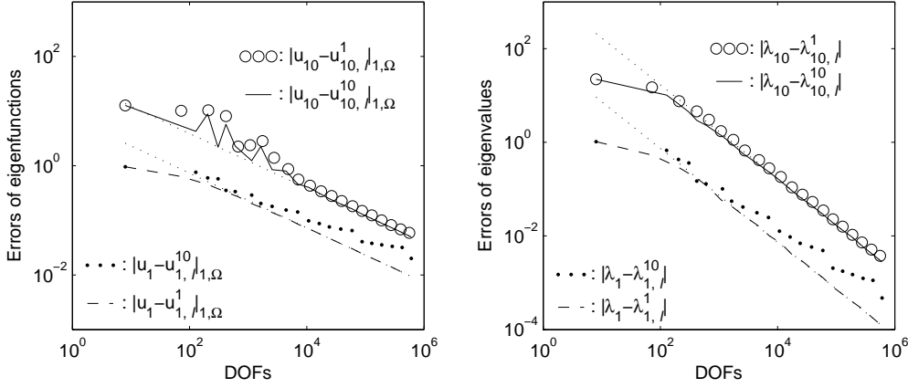
Figure 3. Convergence rates of u_{10,\ell}^1, u_{10,\ell}^{10}, u_{1,\ell}^{10}, u_{1,\ell}^1 (left), and \lambda_{10,\ell}^1, \lambda_{10,\ell}^{10}, \lambda_{1,\ell}^{10}, \lambda_{1,\ell}^1 (right) for Example 6.1. Dotted lines give reference slopes -1/2 (left) and -1 (right).
