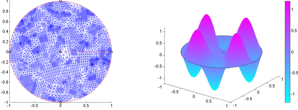
Figure 8. The adaptively refined mesh (left) of 9327 elements and the eigenfunction u_{10,8}^{10} (right) after 8 adaptive iterations for Example 6.2
