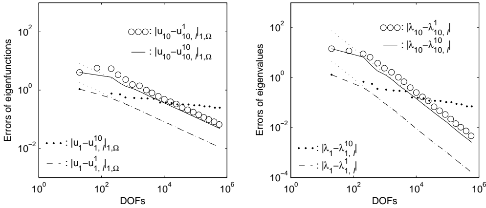
Figure 7. Convergence rates of u_{10,\ell}^1 , u_{10,\ell}^{10} , u_{1,\ell}^{10} , u_{1,\ell}^1 (left), and \lambda_{10,\ell}^1 , \lambda_{10,\ell}^{10} , \lambda_{1,\ell}^{10} , \lambda_{1,\ell}^1 (right) for Example 6.2. Dotted lines give reference slopes -1/2 (left) and -1 (right).
