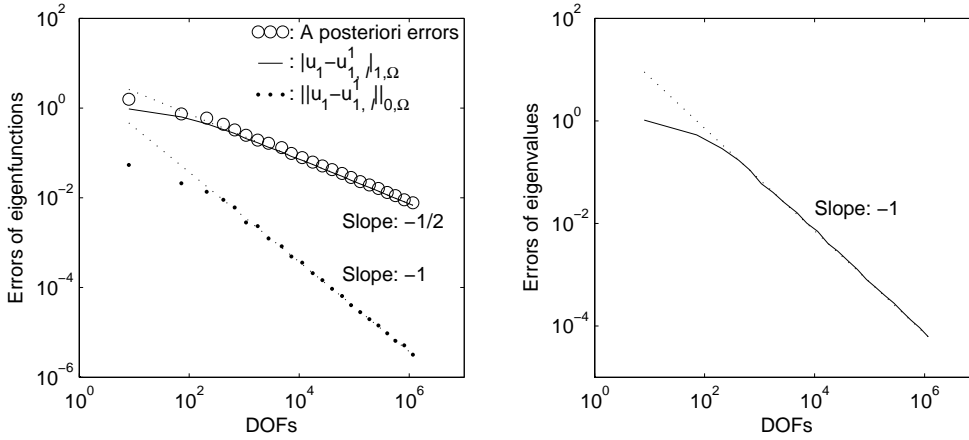
Figure 1. Convergence rates of u_{1,\ell}^1 (left) and \lambda_{1,\ell}^1 (right) for Example 6.1. Dotted lines give reference slopes.
